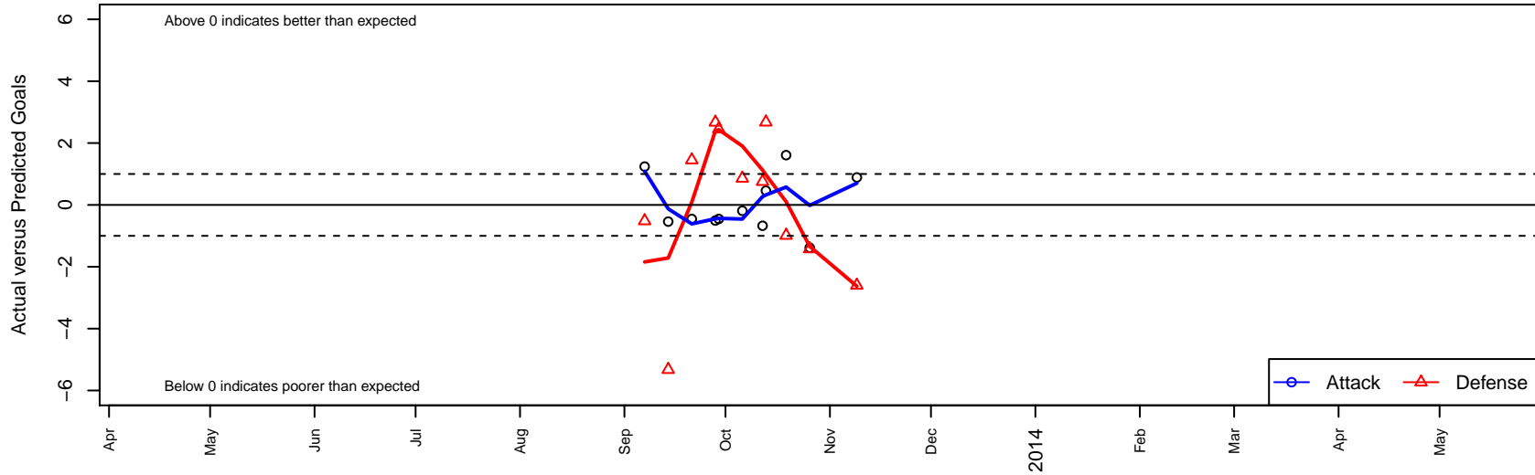
PCFC White B00 Dots are actual minus expected GF (blue circles) and GA (red triangles). Blue line is smoothed change in attack strength. Red is smoothed change in defense strength.
